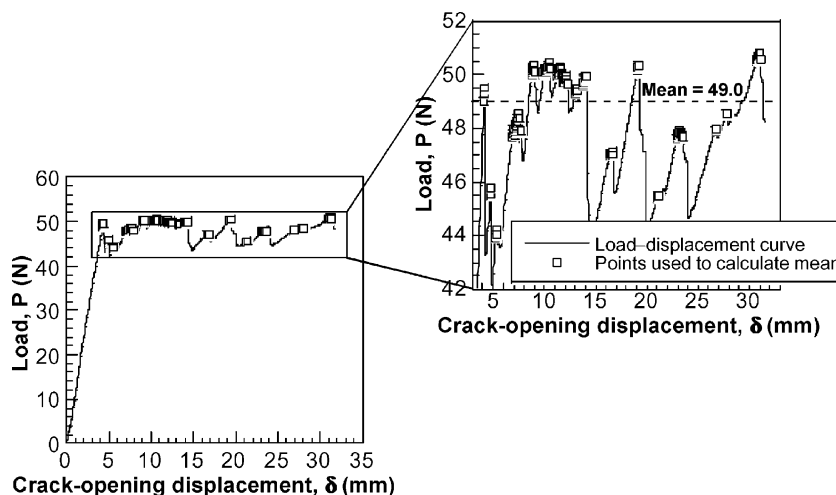
Fig. 5. Data reduction procedure for WTDCB tests to obtain the average fracture toughness from load–displacement data.
